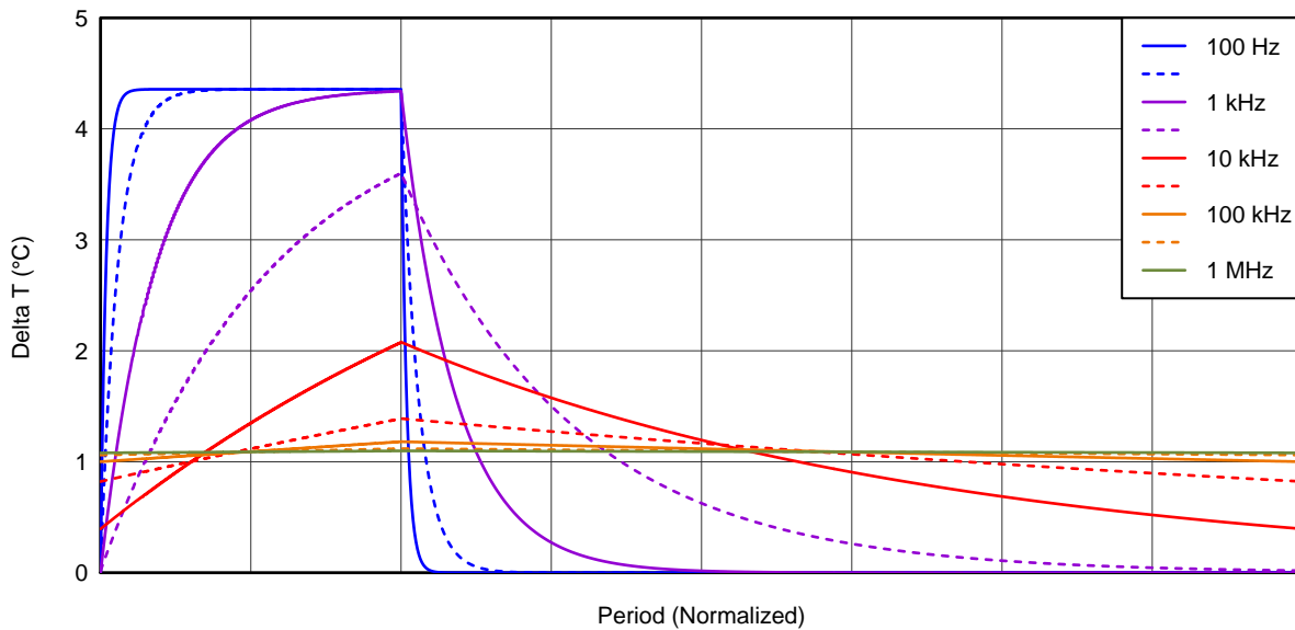
Figure 8. Temperature Over One Cycle for 25% Duty Cycle at Various Frequencies
