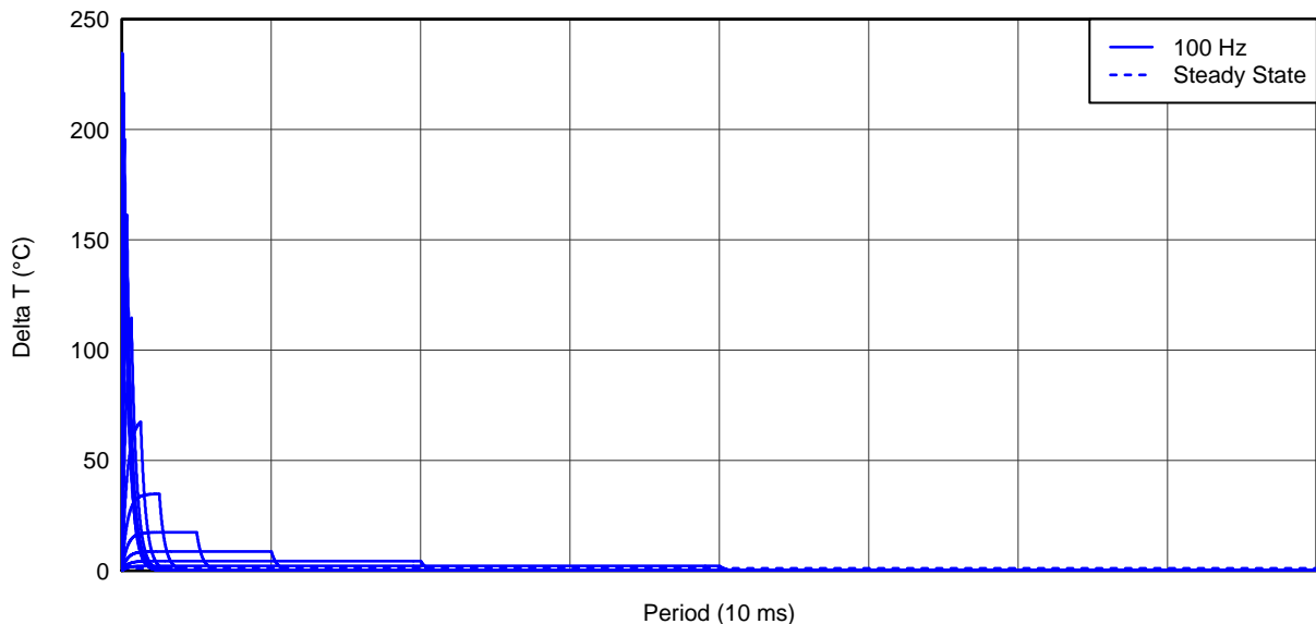
Figure 9. Temperature Over One Cycle for Various Duty Cycles at 100 Hz
