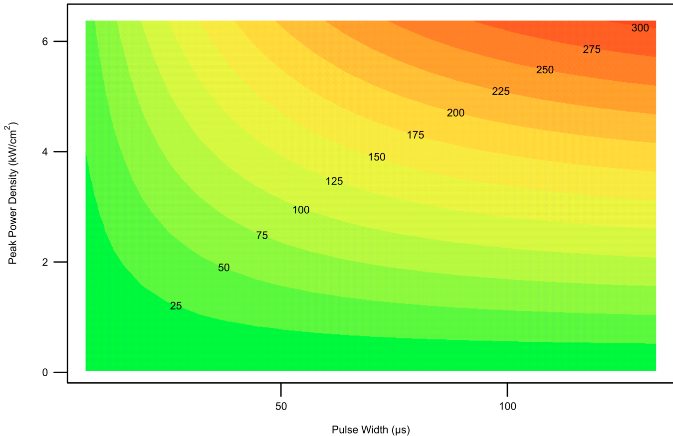
Figure 14. Pixel \Delta T for 13.68 \mu\text{m} Pixel
