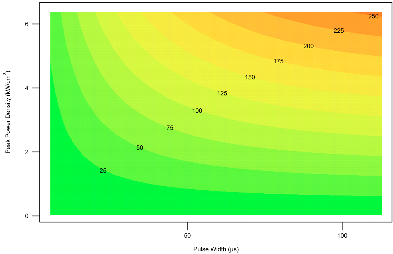
Figure 13. Pixel \Delta T for 10.86 \mu\text{m} Pixel
