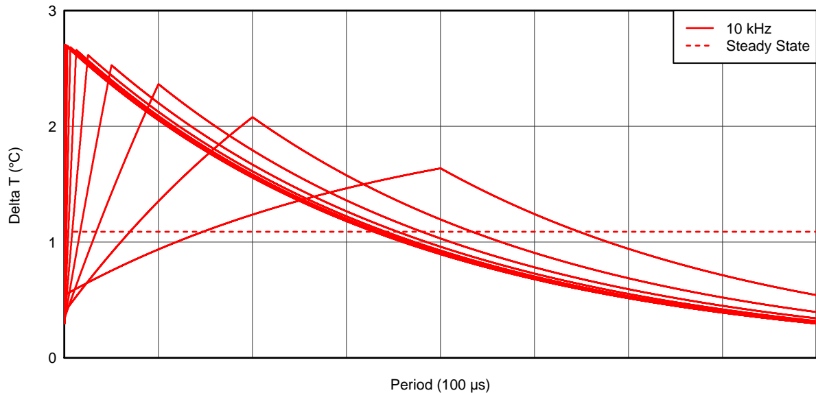
Figure 10. Temperature Over One Cycle for Various Duty Cycles at 10 kHz
