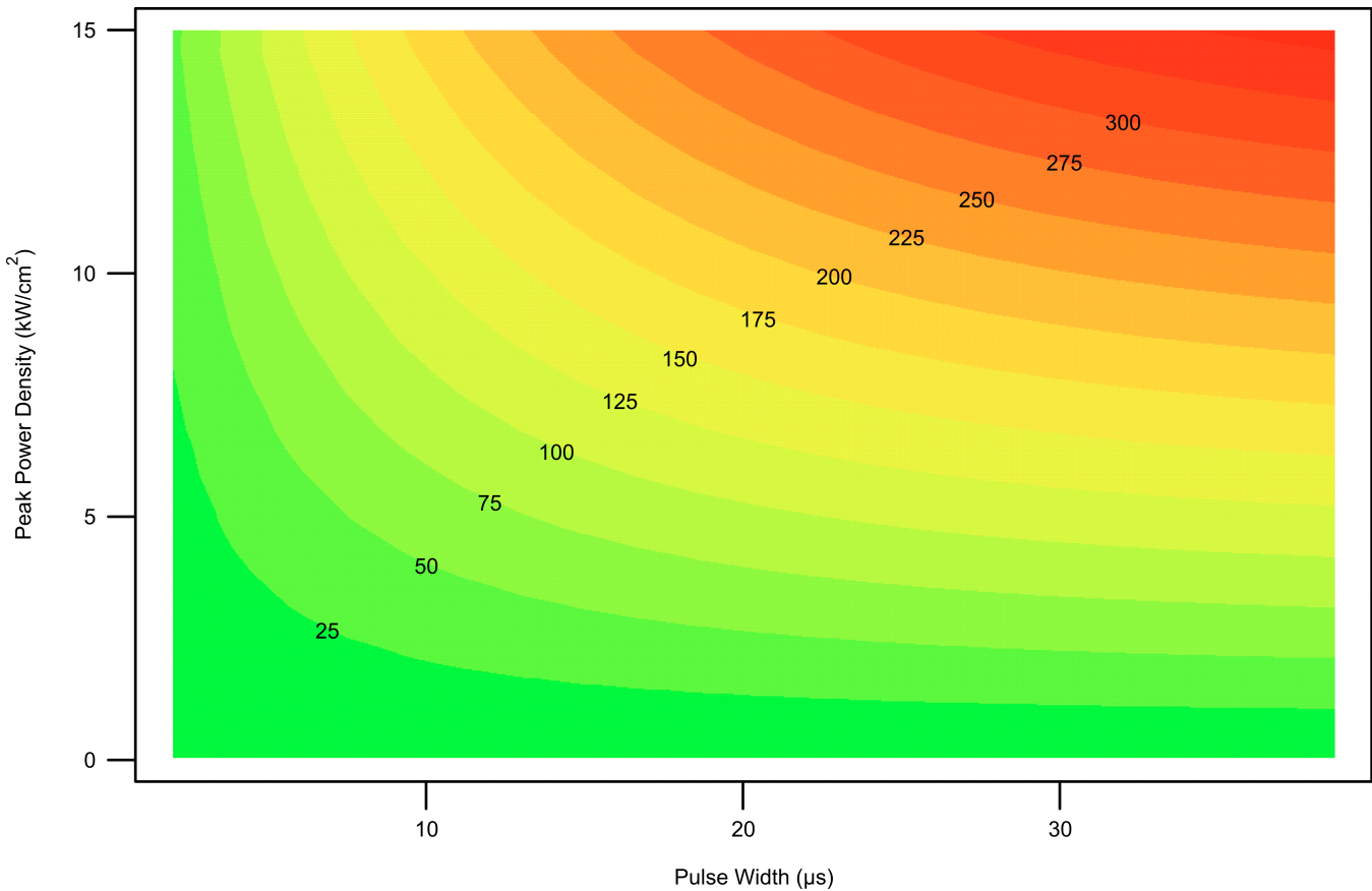
Figure 12. Pixel \Delta T for 7.56 \mu m Pixel
