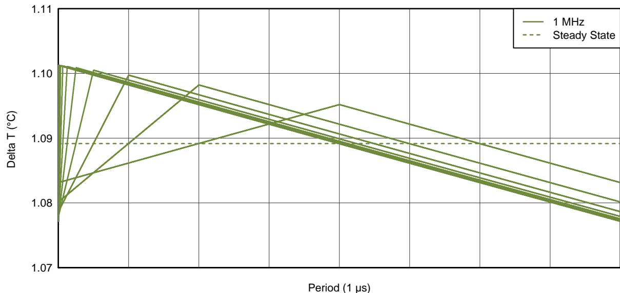
Figure 11. Temperature Over One Cycle for Various Duty Cycles at 1 MHz
