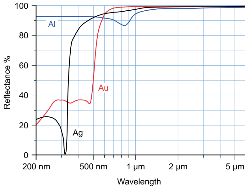
Figure 7. Reflectance vs Wavelength
