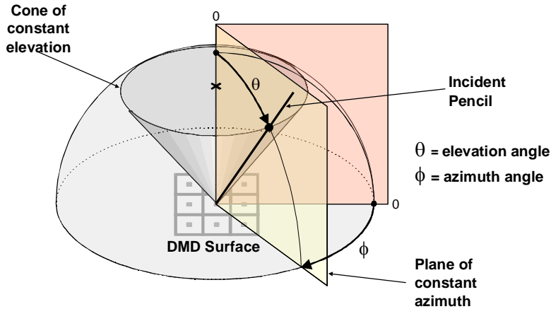
Figure 9. Scattering Incident-Beam Geometry
