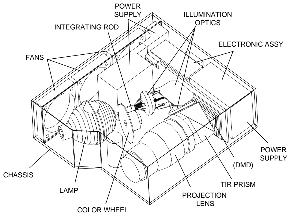
Figure 3. Telecentric TIR Prism Design Layout for Minimum Package Height Due to Projection-Lens Offset
