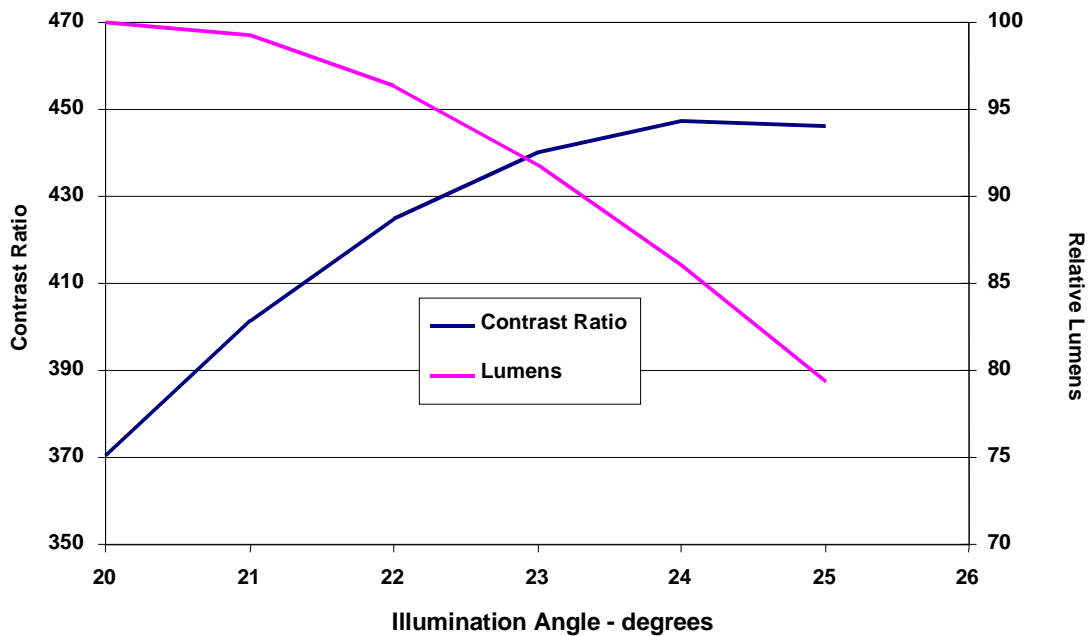
Figure 11. Contrast and Lumens as a Function of Illumination Angle for F/3 Telecentric System (17-um, 10-degree tilt, 0.8-um mirror-ap device)
