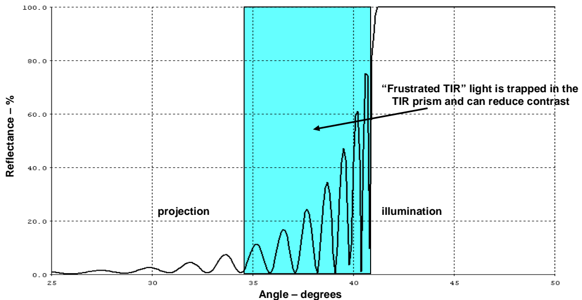
Figure 8. Frustrated TIR in TIR Prism Air Gap Should be Biased Toward Illumination Path
