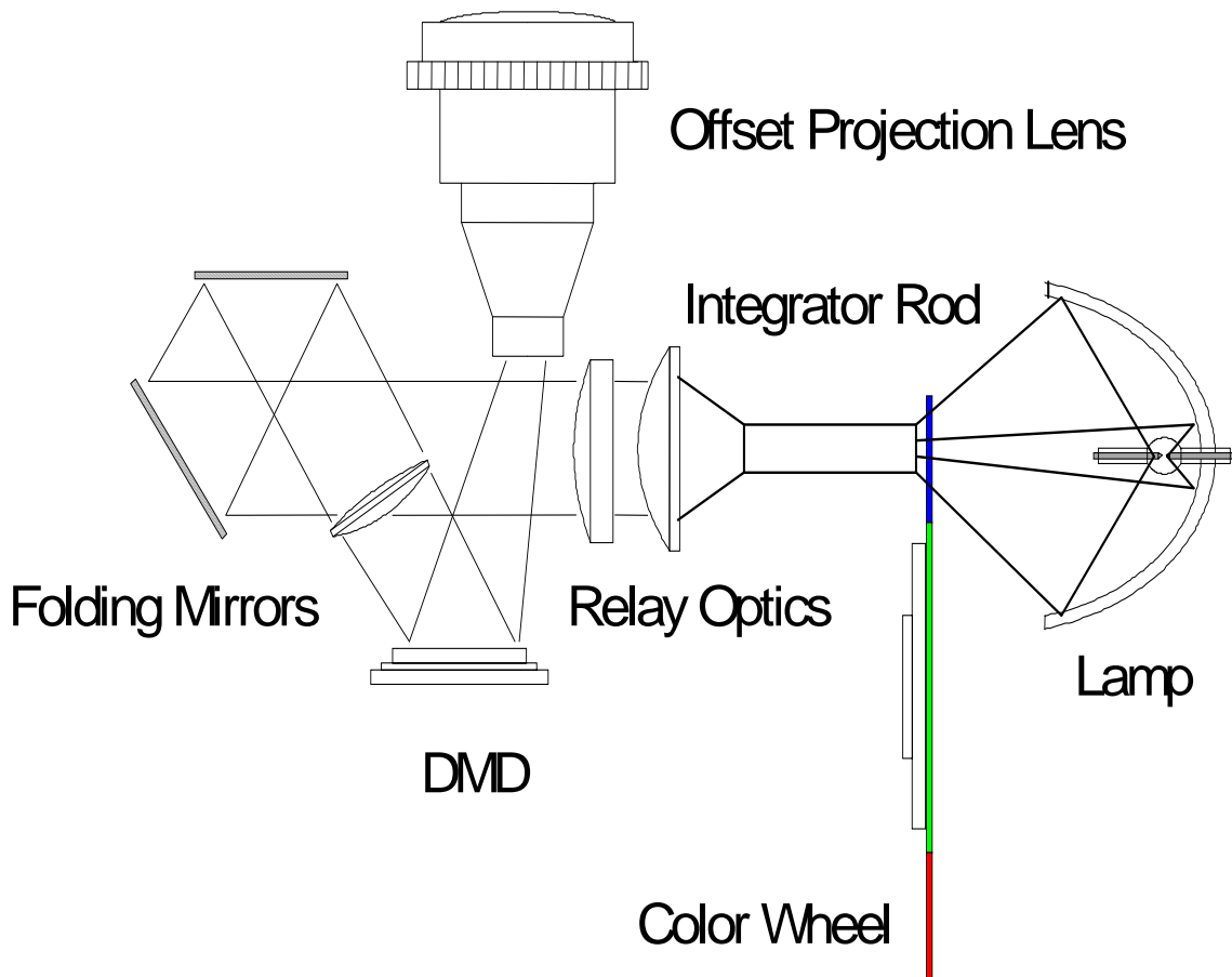
Figure 4. Nontelecentric Optical-System Components
