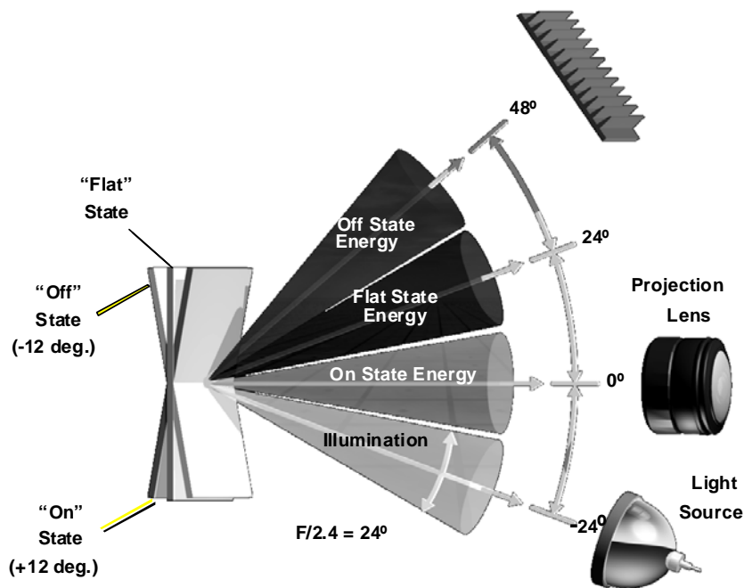
Figure 1. Simplified Optical Function of a 12-Degree-Mirror-Tilt Device
