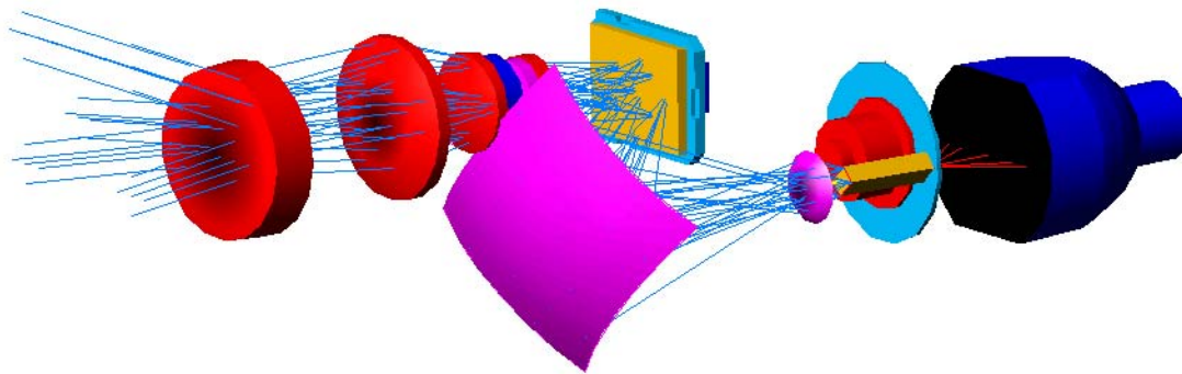
Figure 6. Nontelecentric Optical Layout for Flat Projector Using Reflective and Refractive Illumination Elements (Isometric View)
